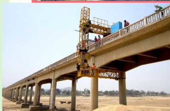
Mobile Bridge Inspection Unit
