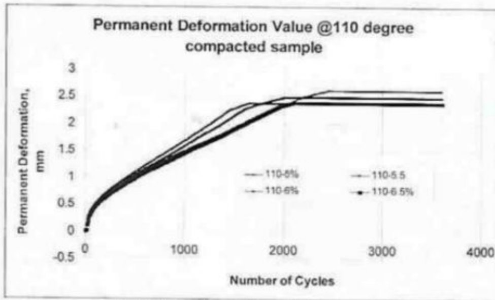
Fig 4 e. Creep value at different binder content
