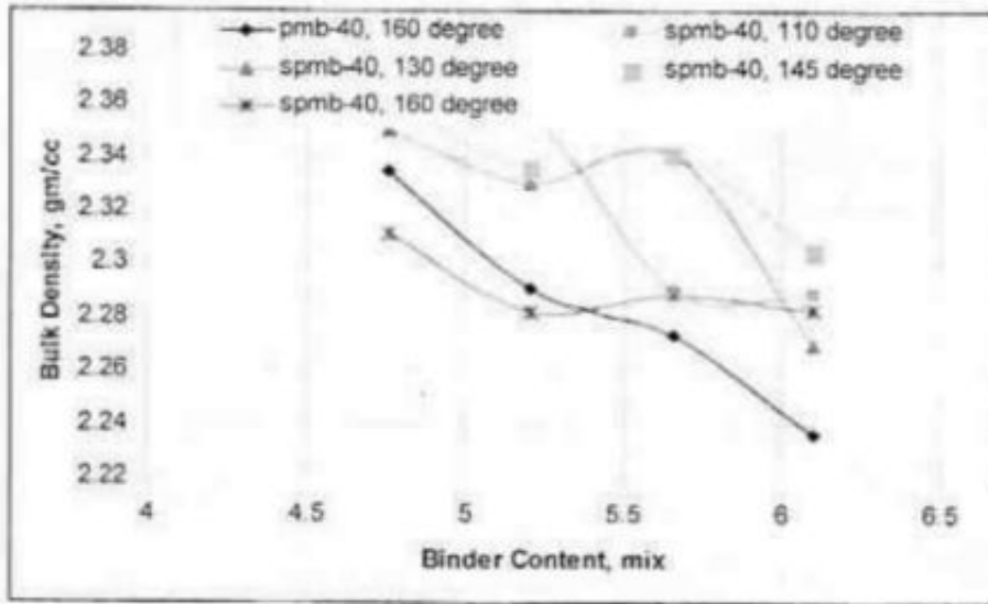
Figure 2 a: Volumetric Properties of SMA Mixture
