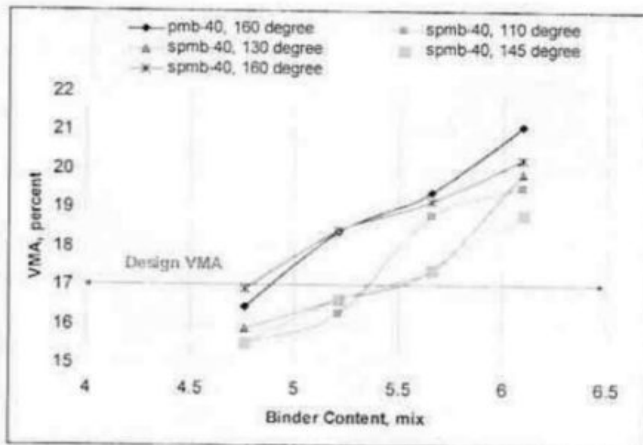
Figure 2 c: Volumetric Properties of SMA Mixture
