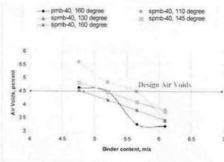
Figure 2 b: Volumetric Properties of SMA Mixture
