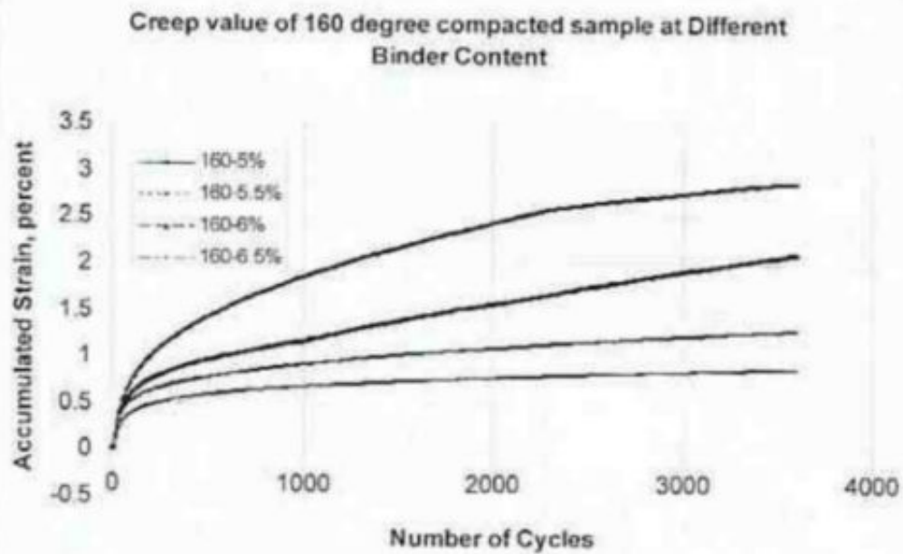
Fig 4 c. Creep value at different binder content
