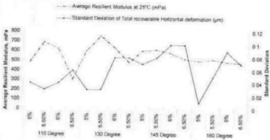
Fig 3 b. The Resilient Modulus of the mixes at various temperature
