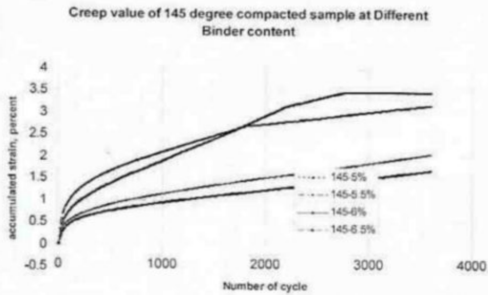
Fig 4 c. Creep value at different binder content
