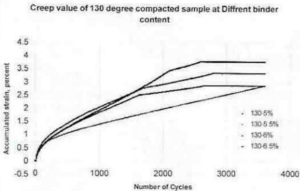
Fig 4 b. Creep value at different binder content
