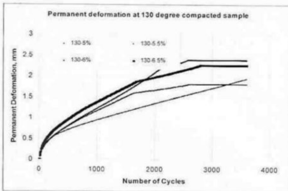
Fig 4 f. Creep value at different binder content
