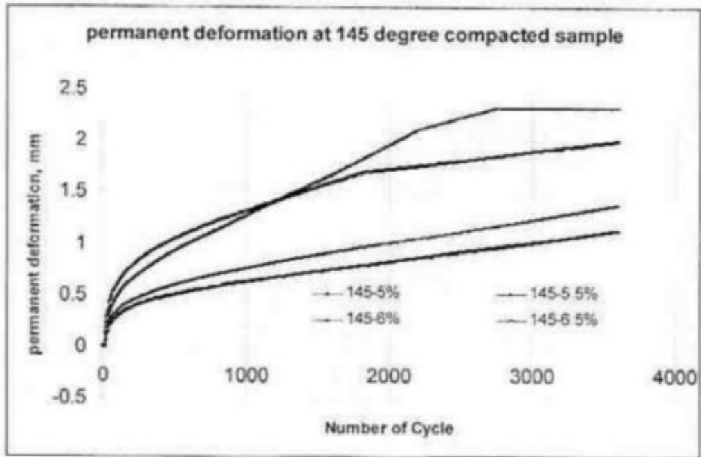
Fig 4 g. Creep value at different binder content
