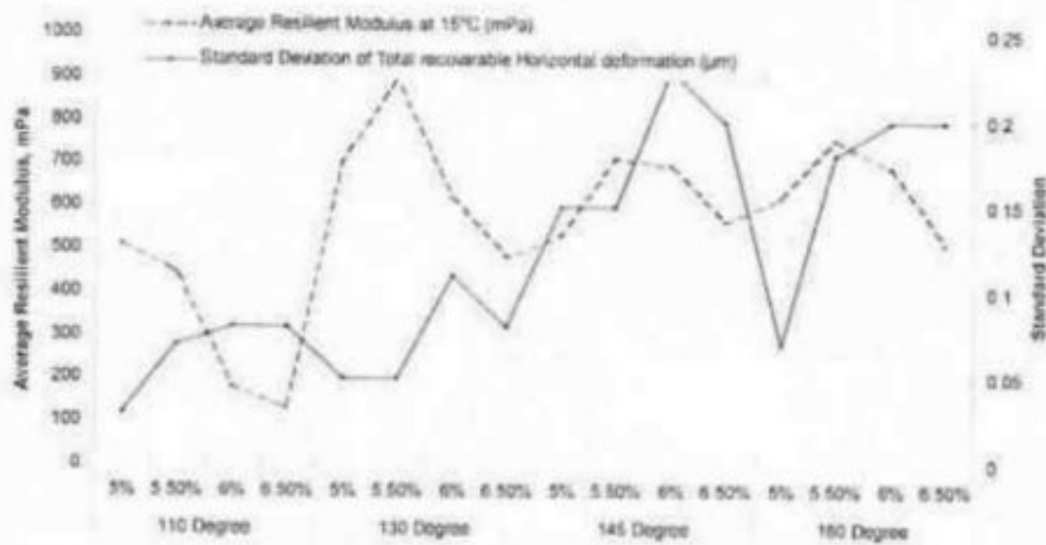
Fig 3 a. The Resilient Modulus of the mixes at various temperature
