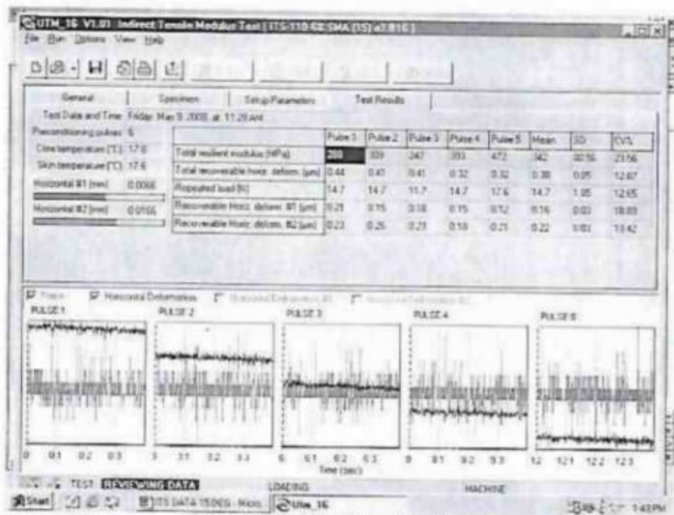
Fig 3 d. Indirect tensile modulus test
