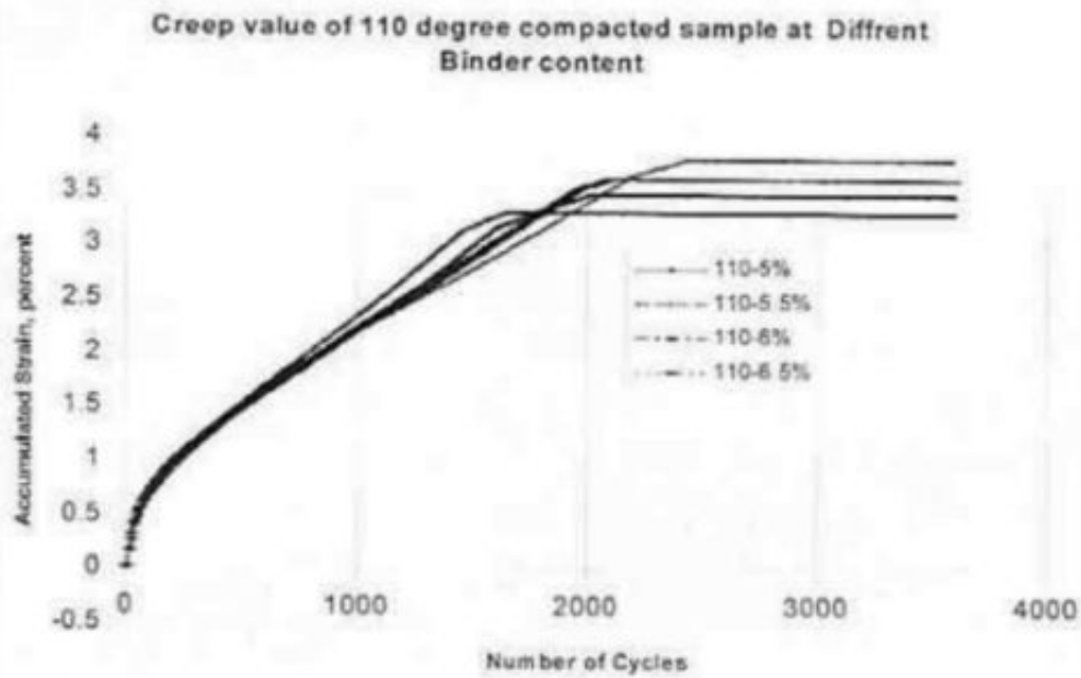
Fig 4 a. Creep value at different binder content
