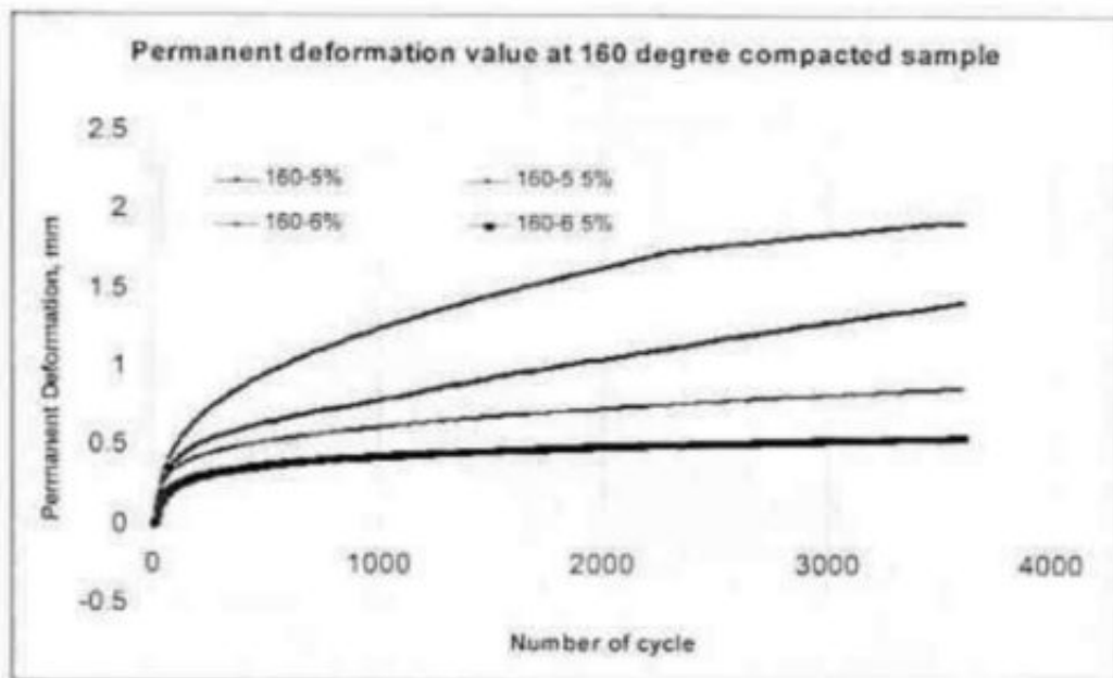
Fig 4 h. Creep value at different binder content
